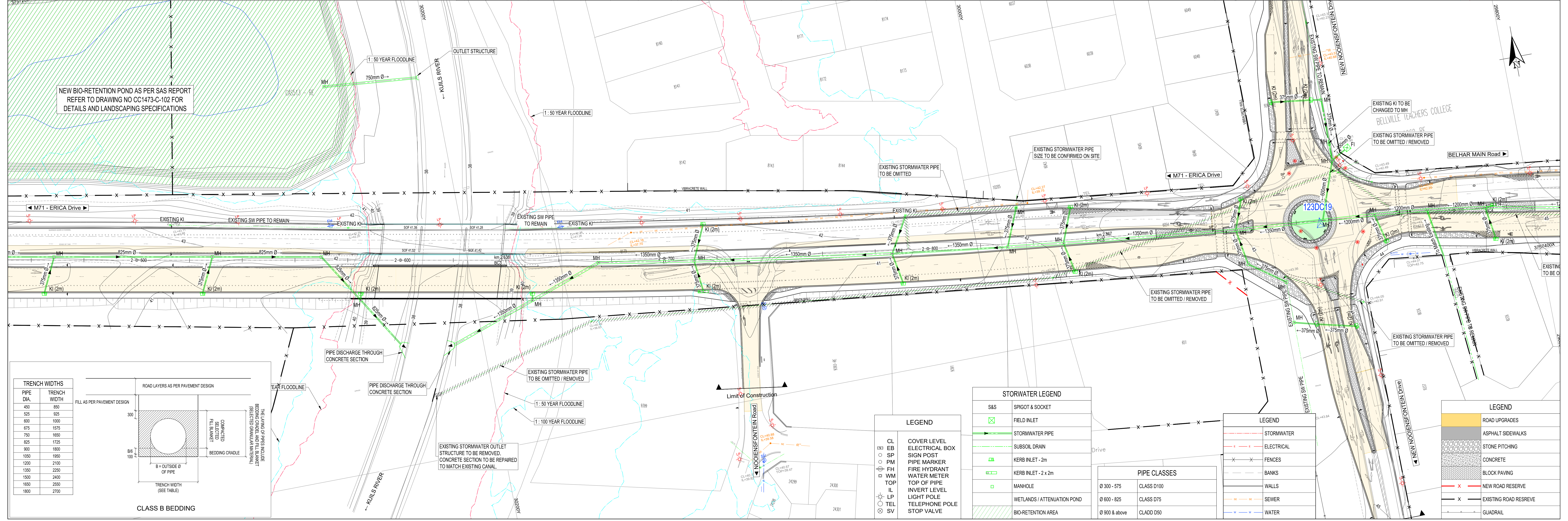
TYPICAL M71 ERICA DRIVE - PHASE 1 DUAL CARRIAGEWAY SECTION FROM KM 1.700 TO END
