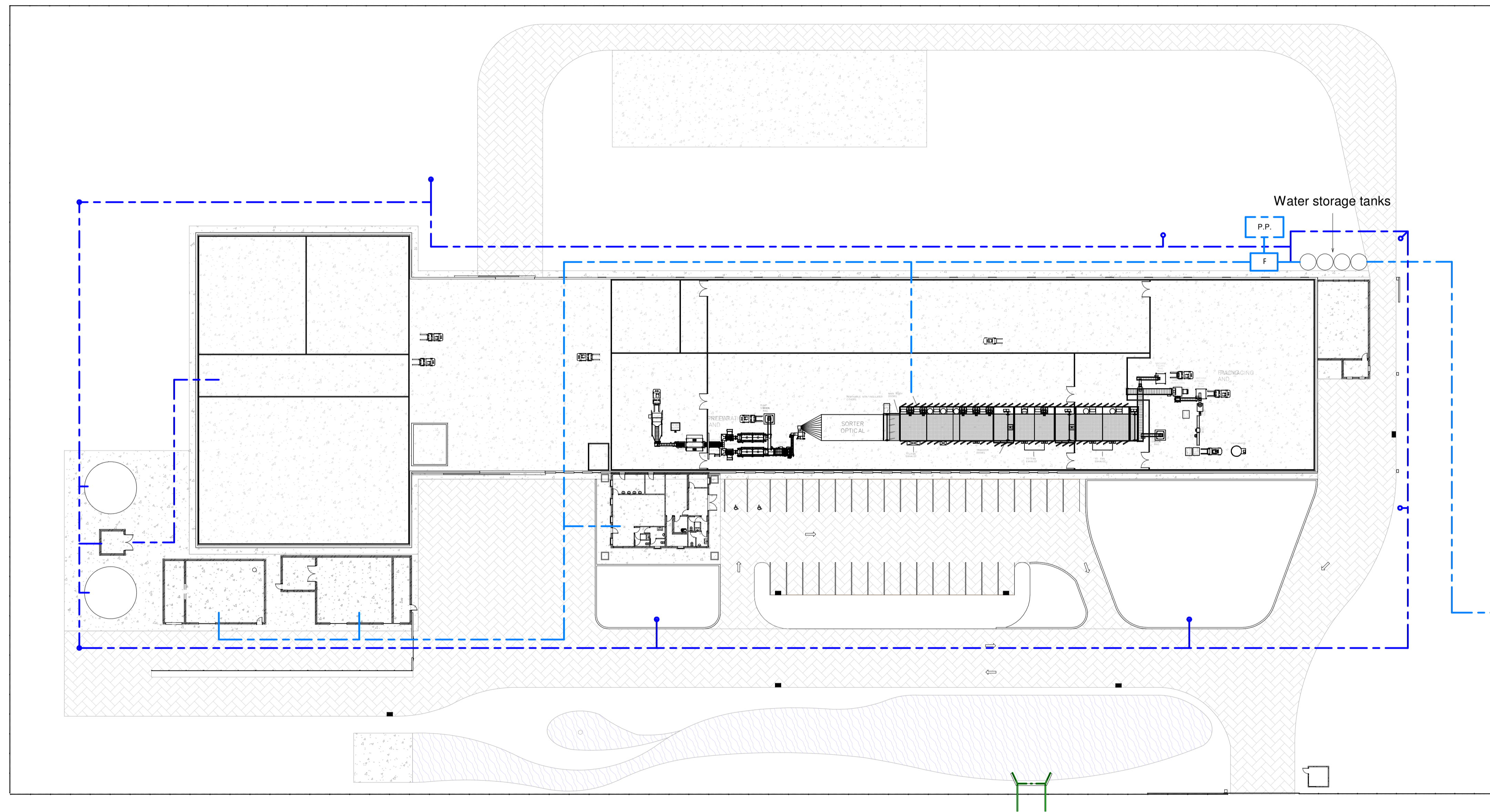
1 Water Reticulation Schematic 1 : 400
